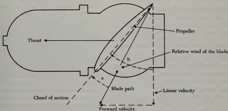
FIGURE 7-6. Propeller forces.
